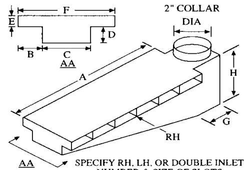
SLOTTED EXHAUST HOOD
