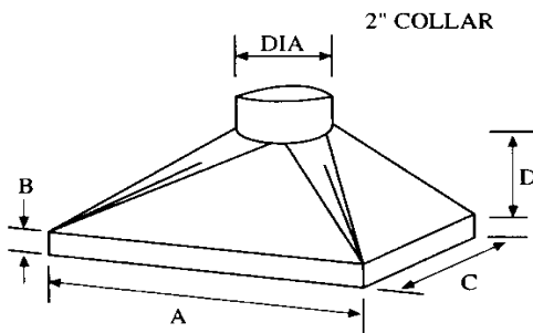
CANOPY EXHAUST HOOD
