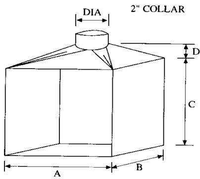
OPEN EXHAUST HOOD
