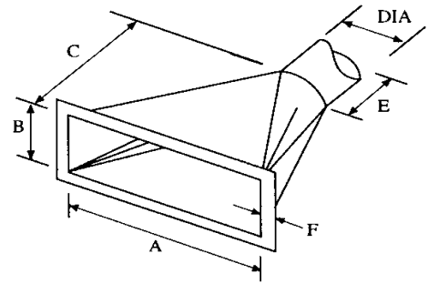
FLANGED OPEN EXHAUST HOOD
