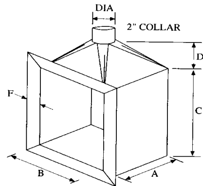
FLANGED OPEN EXHAUST HOOD
