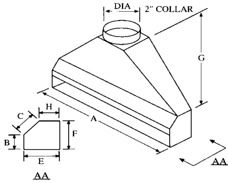
SLOTTED EXHAUST HOOD
