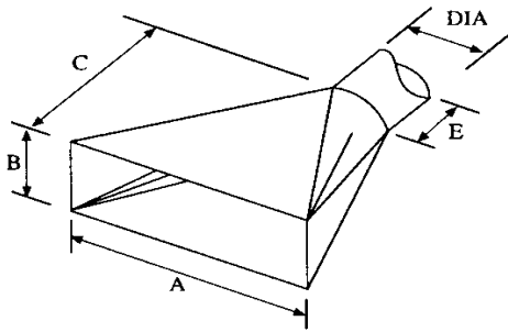
OPEN EXHAUST HOOD
